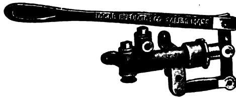
FIG. 202a.—Typical Hand Pump for Steam Carriage Use. This style of pump is used on a large number of American steam carriages, and is an indispensable adjunct—its object being to supply water to the boiler when, for any reason, the automatic pump fails to work. The particularly advantageous feature is the jointed hand lever, which may be bent back out of the way, when not in use, and readily brought to the driver's hand, when necessary.
